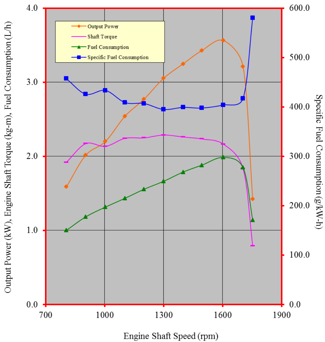
Figure 3. Performance characteristic curves of the BRIGGS & STRATTON, VANGUARD 13H362 gasoline engine w/ gear reduction
