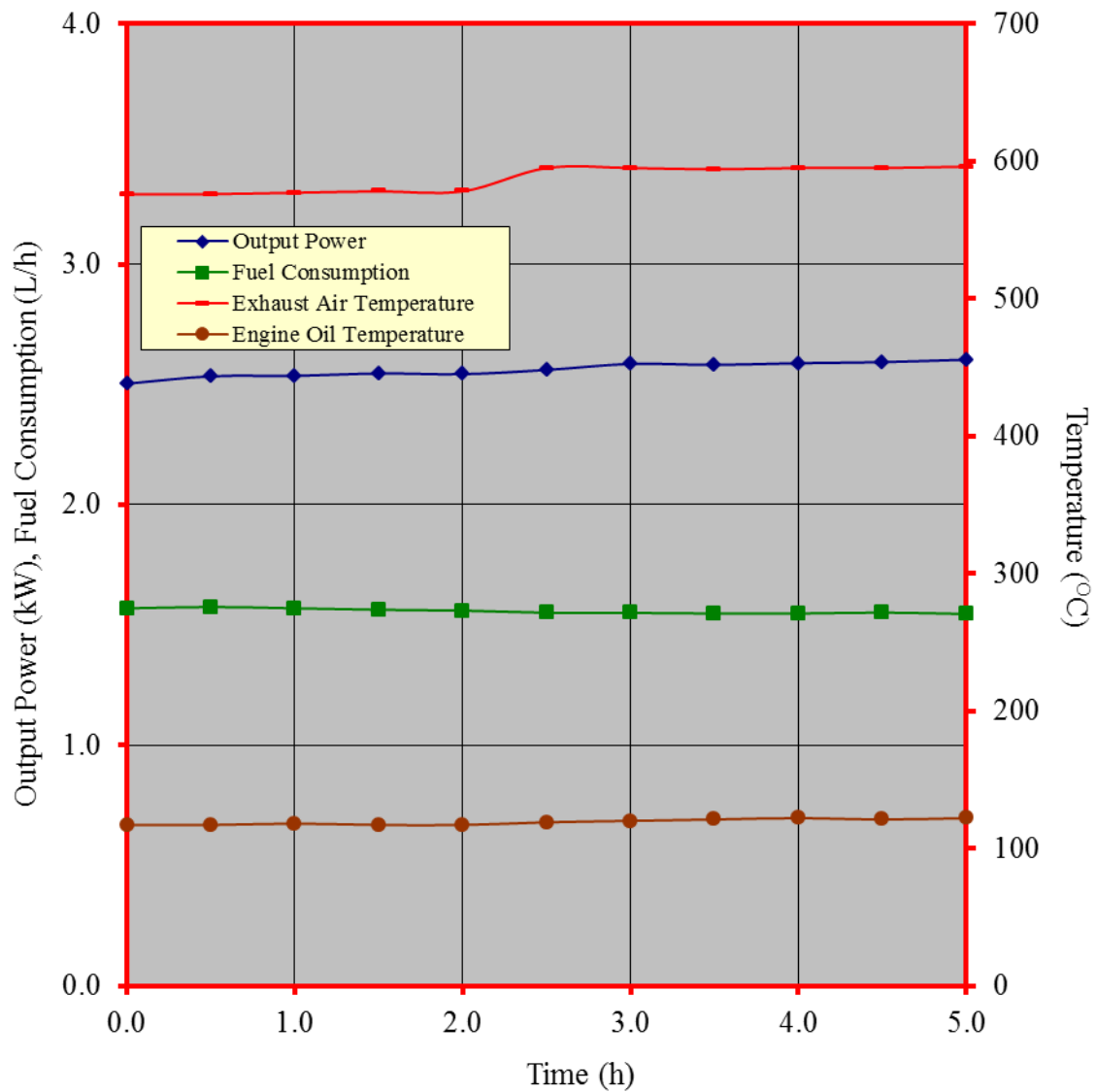
Figure 4. Performance characteristic curves during the continuous running test of the BRIGGS & STRATTON, VANGUARD 13H362 gasoline engine w/ gear reduction
